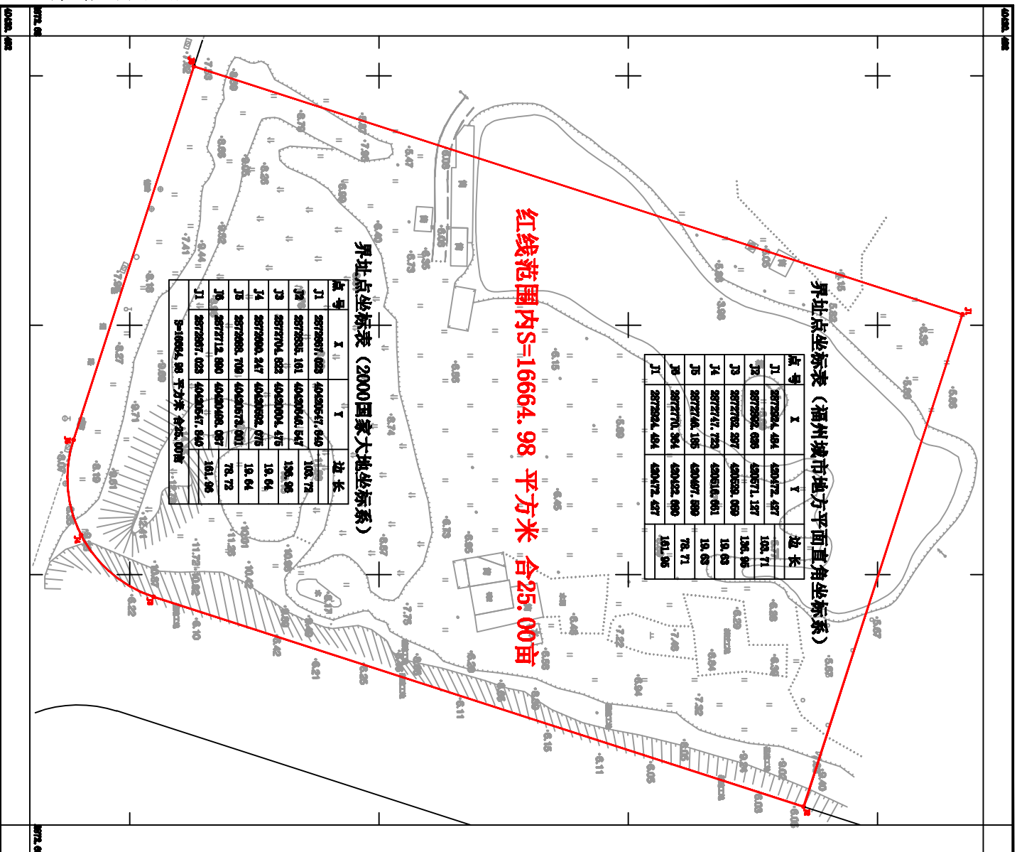
两园南LYN-A-05地块选址红线图 2872.68-40420.49
